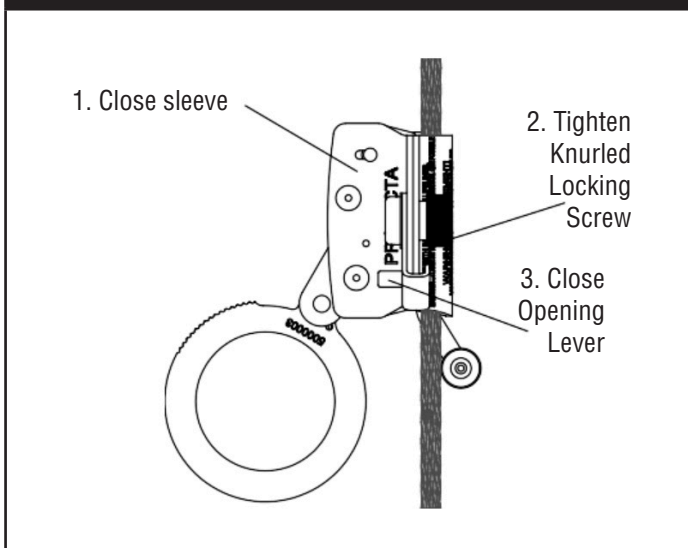
FIGURE 10 - ATTACHING TO LIFELINE
