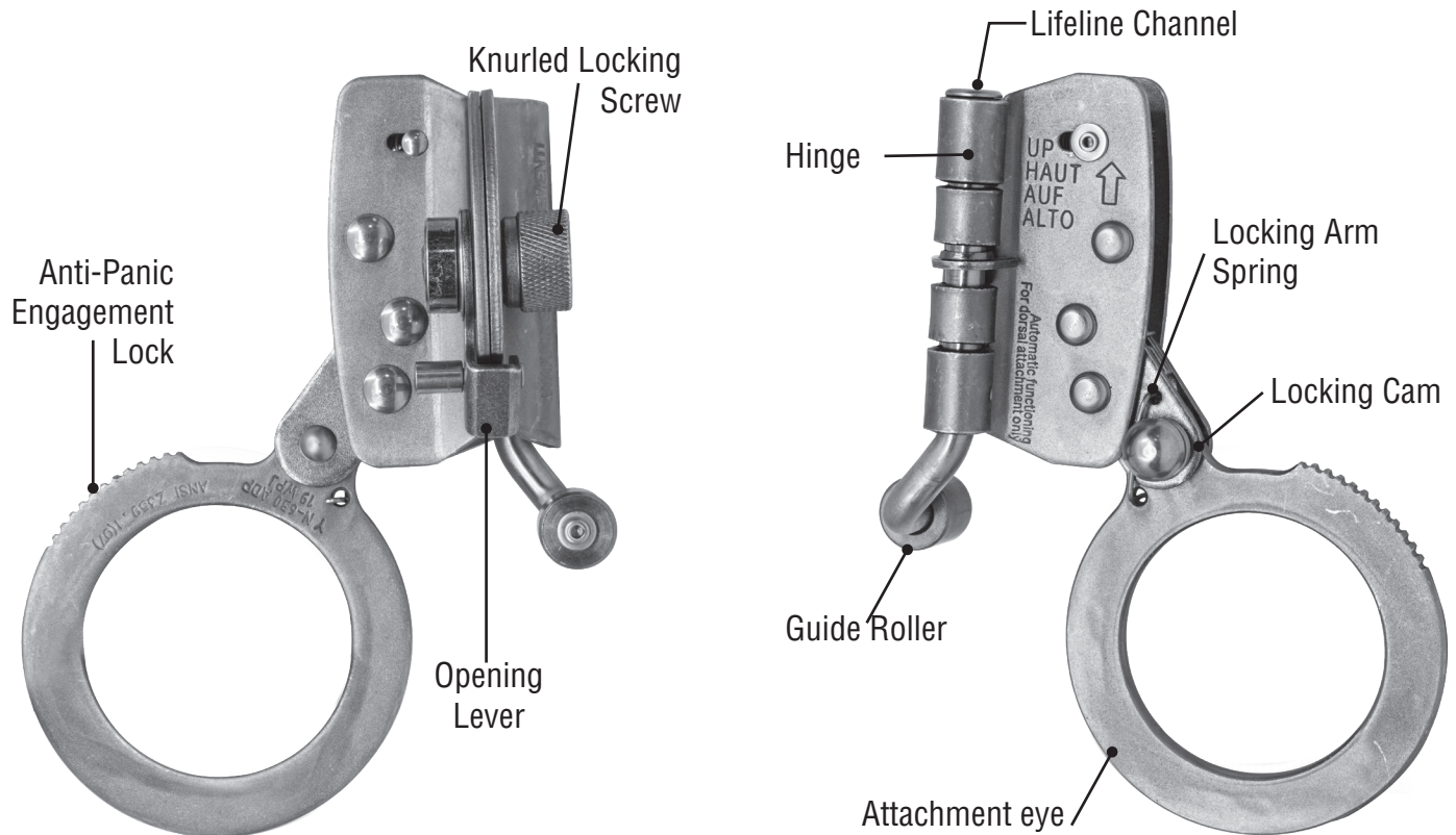
FIGURE 1 - SYNTHETIC ROPE GRAB
